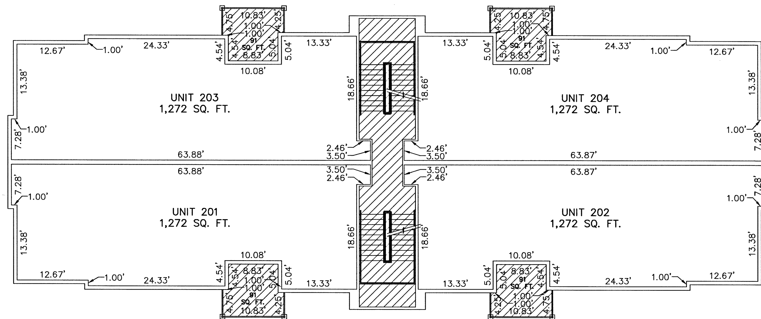
2ND LEVEL
