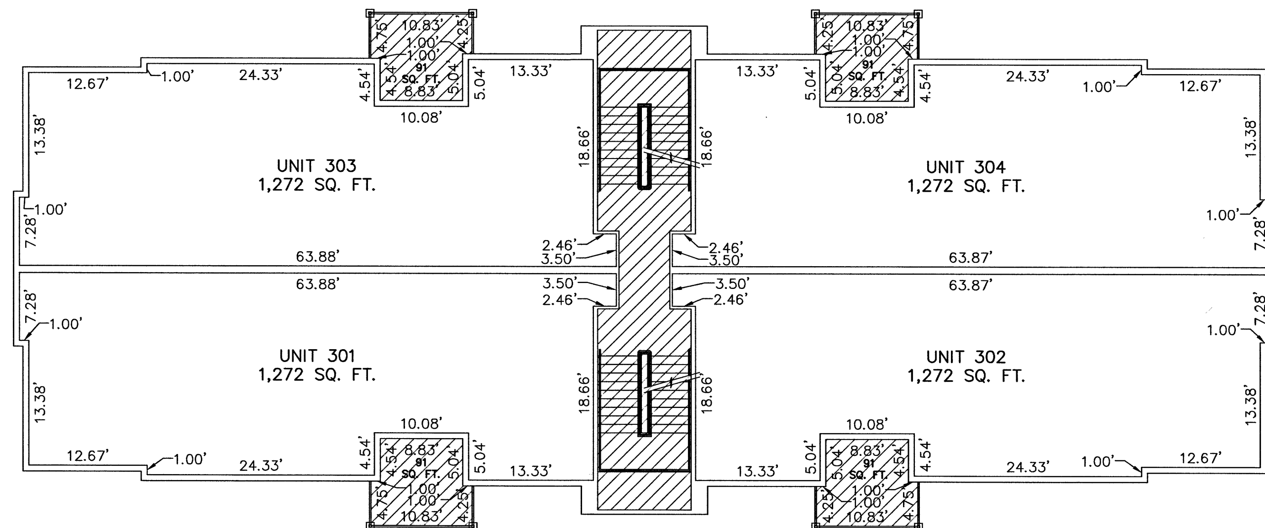
3RD LEVEL
